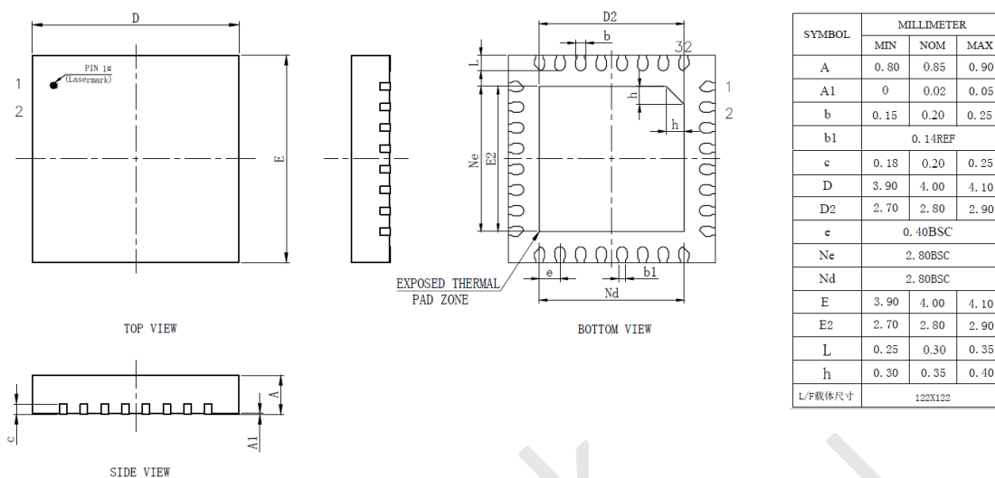
Figure 7-1 TWS200G Package
