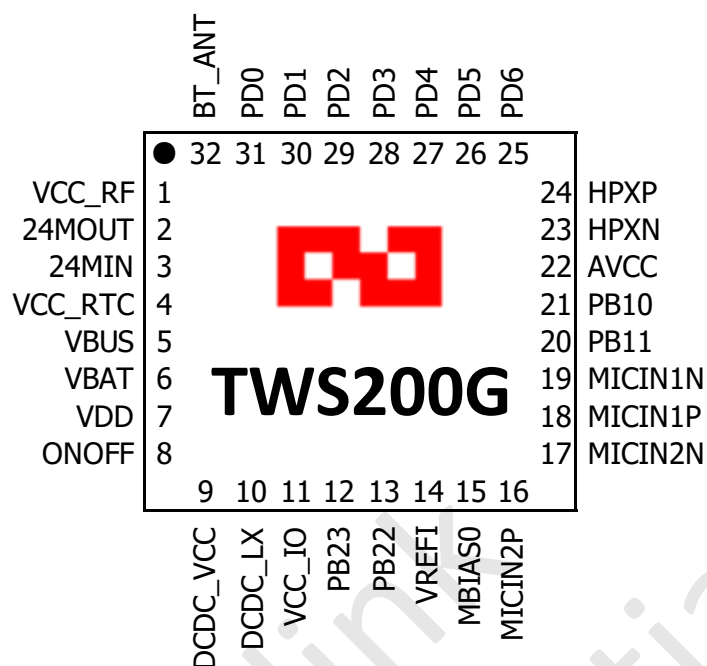
Figure 4-1 TWS200G Pinout
