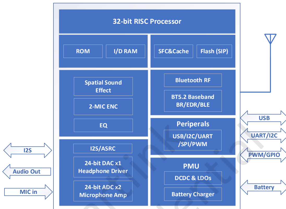
Figure 3-1 TWS200G Block Diagram
